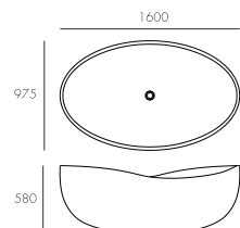
TUB-5001 Size: L x W x H 1600X975X580MM N. W: 170KG
