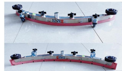
弧形铸铝易装卸水扒胶条可双向使用 Arc cast aluminum water wiper easy up and down,the strips can be used in both directions
